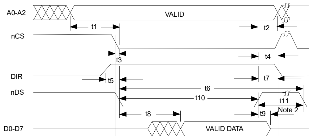
FIGURE 8-8: NON-MULTIPLEXED BUS, 68XX-LIKE CONTROL SIGNALS; READ CYCLE
