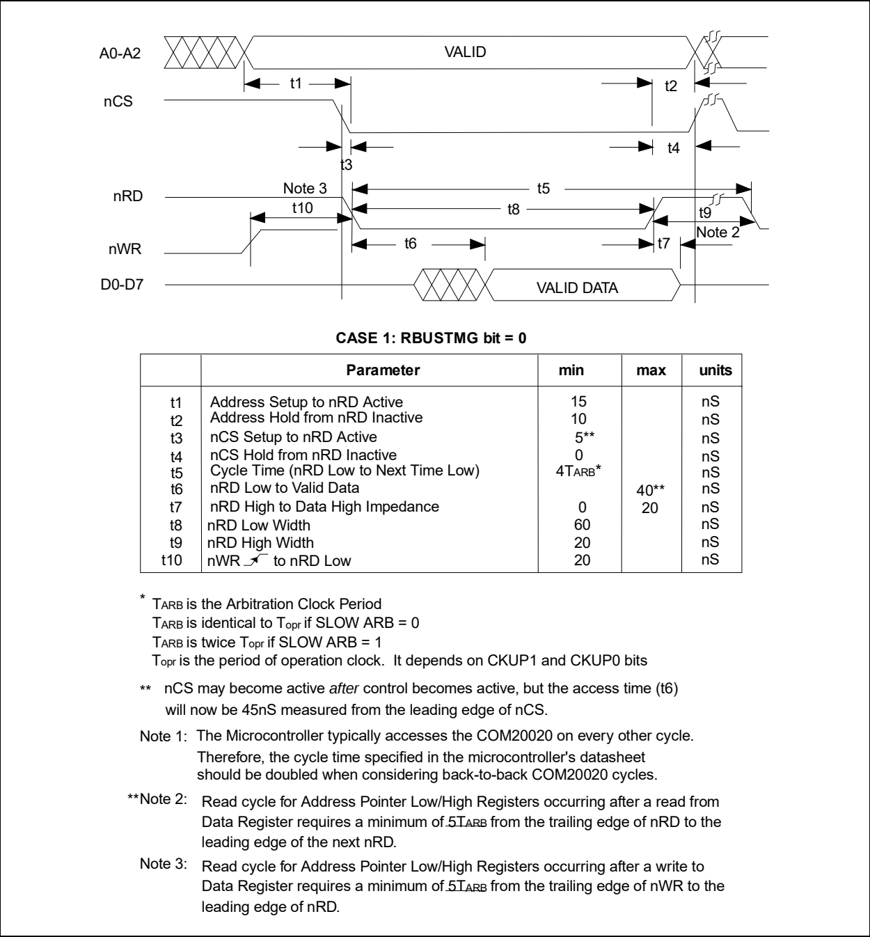
FIGURE 8-5: NON-MULTIPLEXED BUS, 80XX-LIKE CONTROL SIGNALS; READ CYCLE
