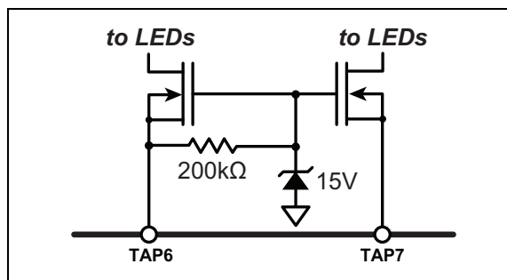
FIGURE 3-4: Power Boost.
