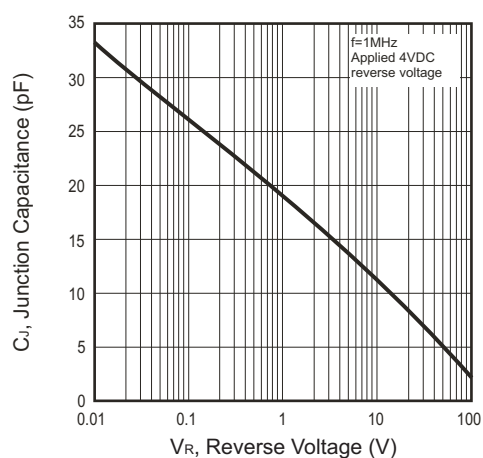
Fig.3 Junction Capacitance
