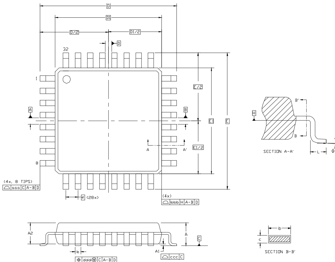
Figure 3.11. LQFP-32 Package Diagram
