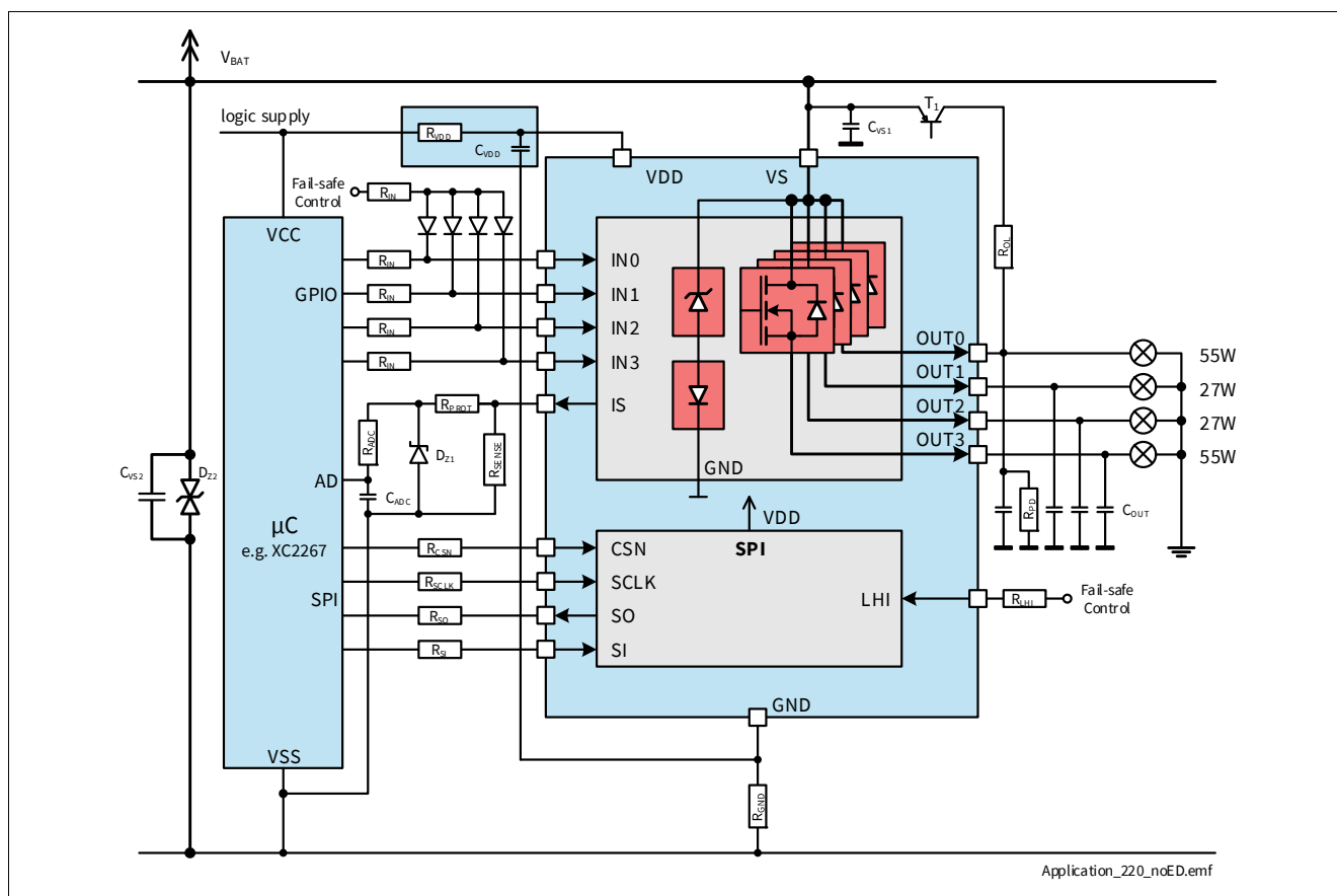
Figure 46 Application Diagram
