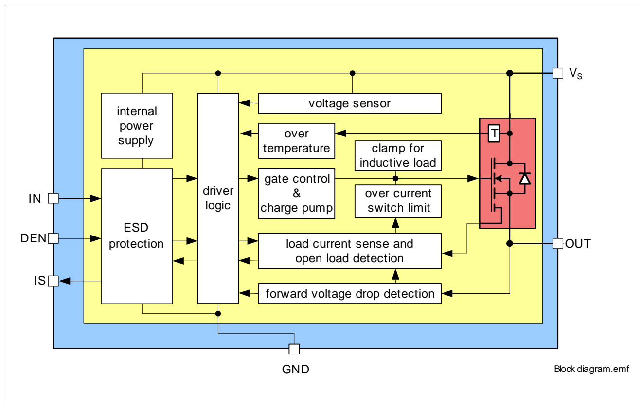
Figure 1 Block Diagram for the BTS5020-1EKA
