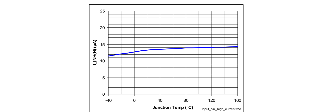
Figure 51 Input Current High Level I_{IN(H)} = f(T_J; V_S)
