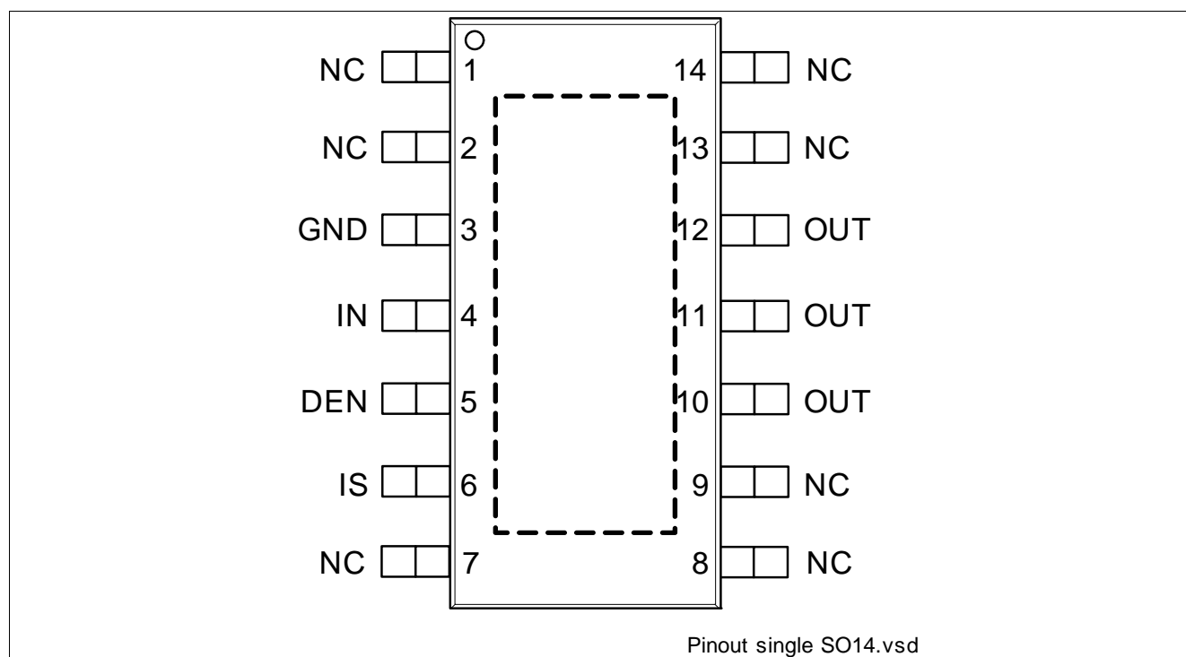
Figure 2 Pin Configuration
