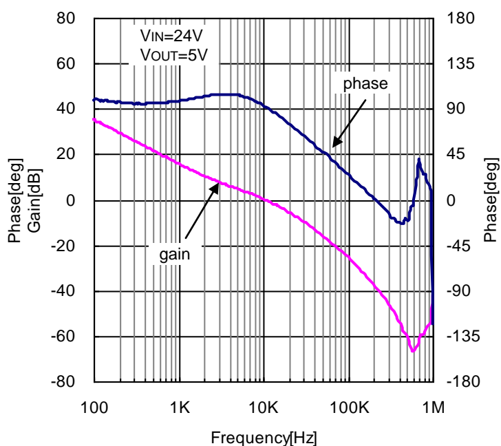
Figure 38. Loop Response (VIN=24V, VOUT=5V, IOUT=2.5A, COUT=Ceramic22μF × 2)
