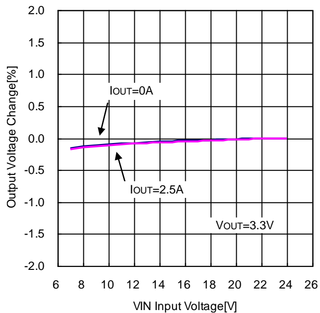
Figure 31. VOUT Line Regulation
