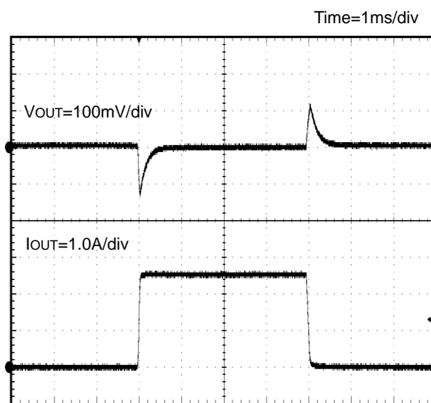
Figure 40. Load Transient Response IOUT=0A – 2.5A (VIN=24V, VOUT=5.0V, COUT=Ceramic22μF × 2)
