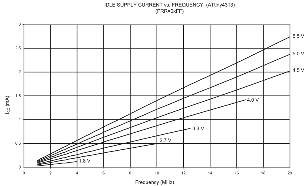
Figure 23-55. Idle Supply Current vs. Frequency (1 - 20 MHz)
