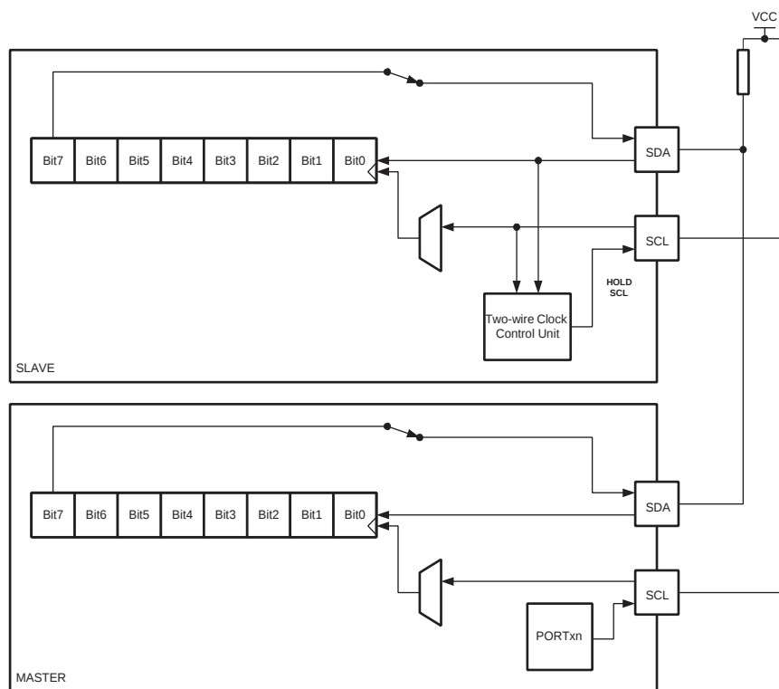
Figure 16-4. Two-wire Mode Operation, Simplified Diagram
