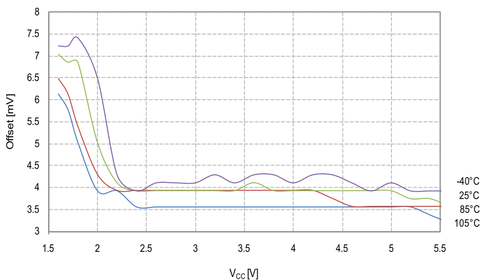
Figure 26-59. Analog Comparator Offset vs. V_{CC} ( V_{IN} = 1.1V )
