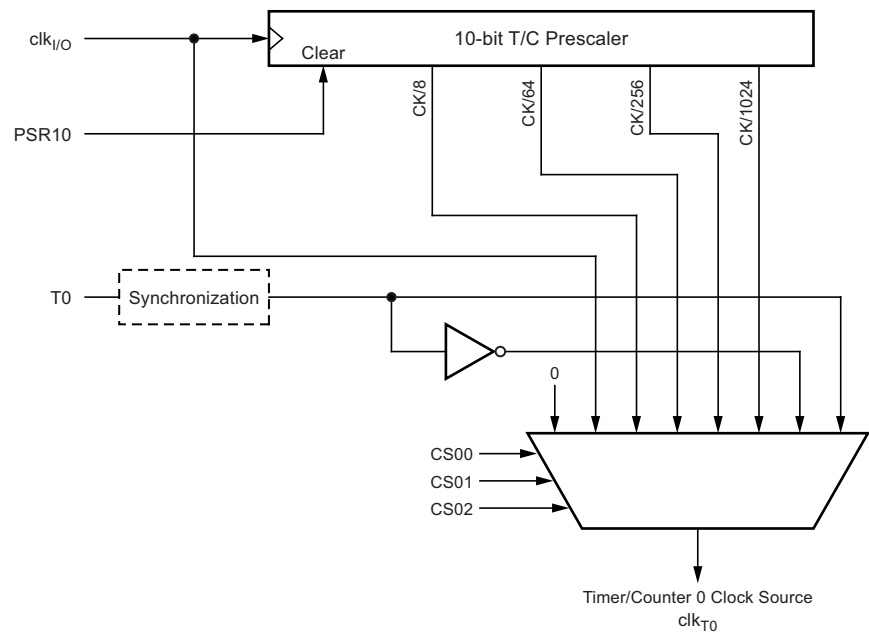
Figure 15-2. Prescaler for Timer/Counter0
