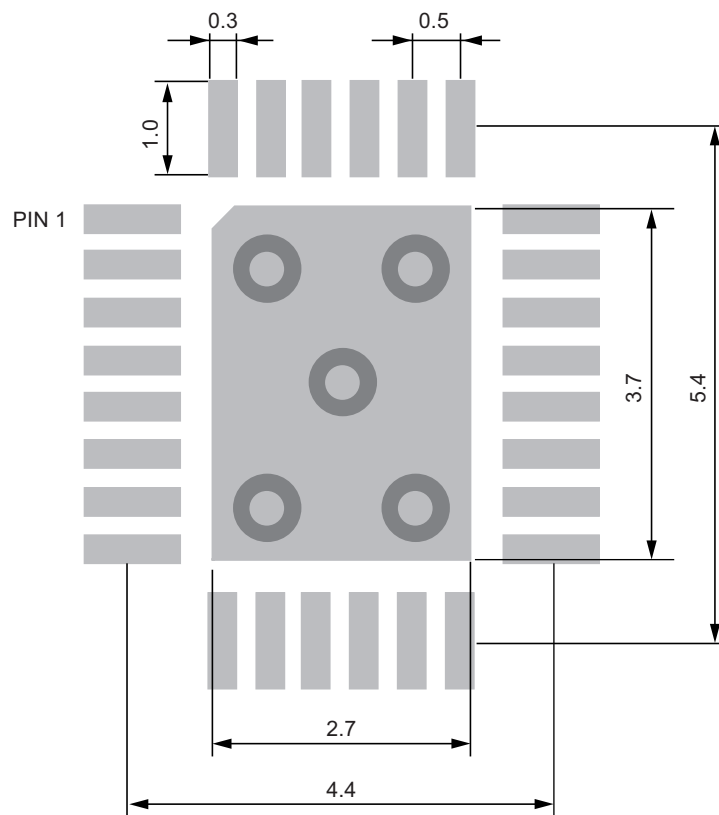
Figure 8-4. Recommended Footprint
