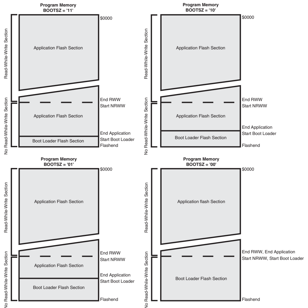
Figure 73. Memory Sections (1)
