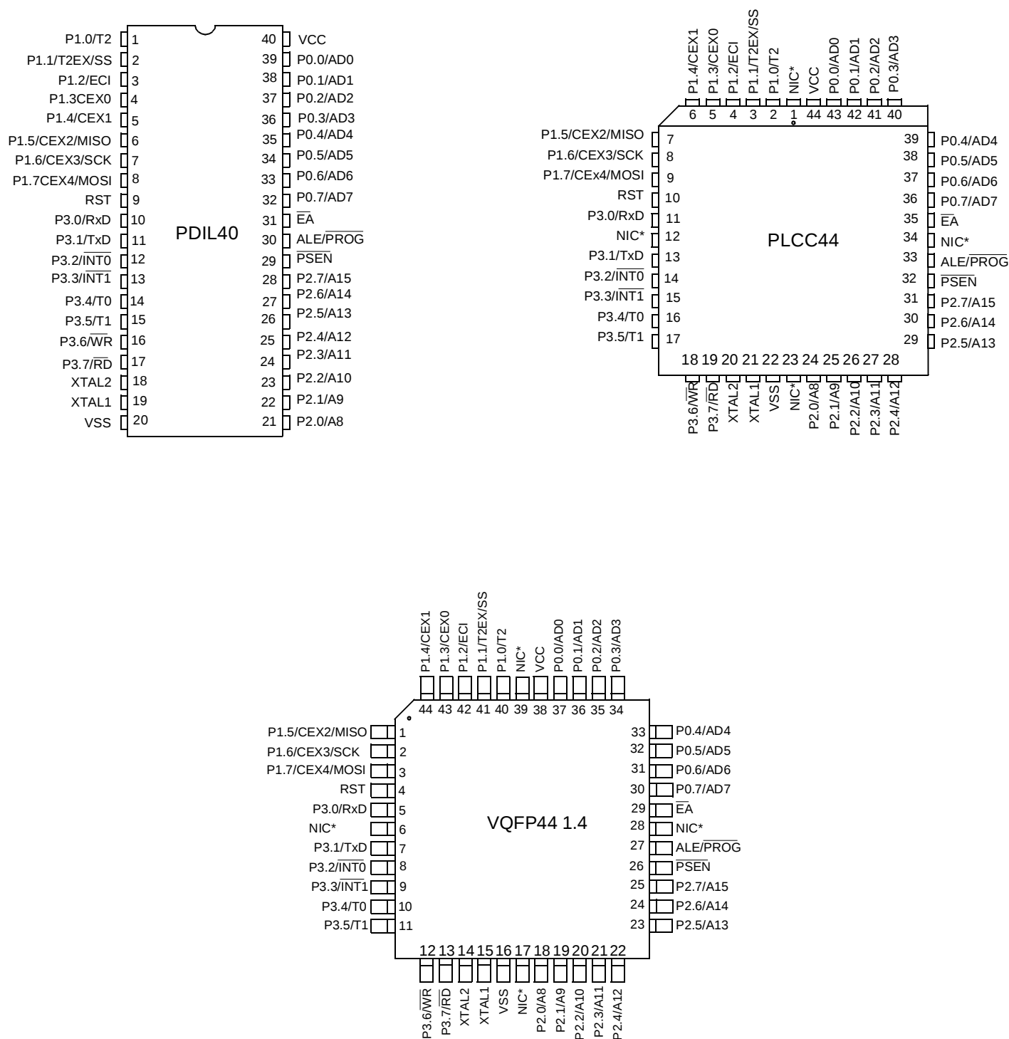
Figure 2. Pin Configurations
