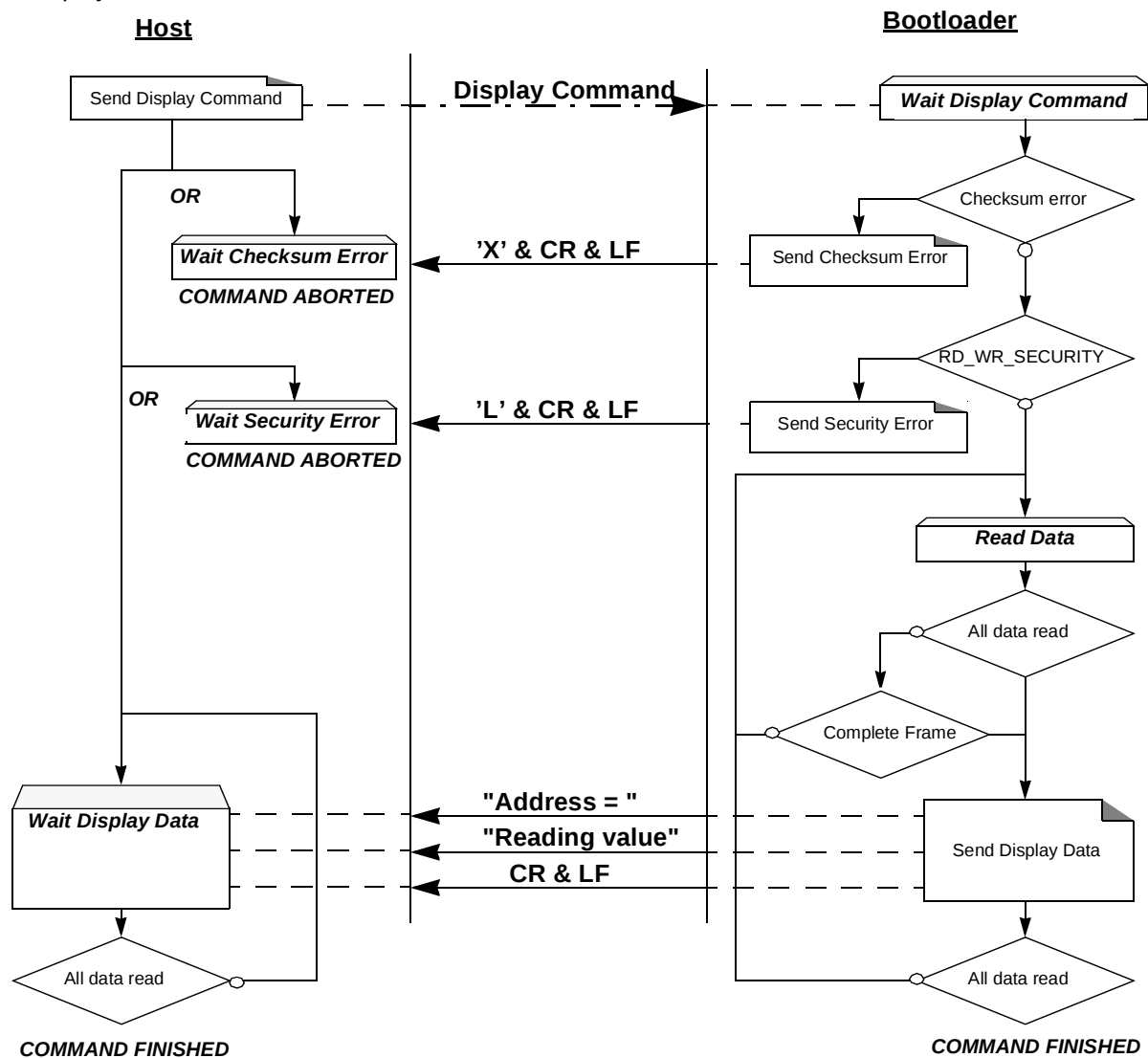
Figure 44. Display Flow
