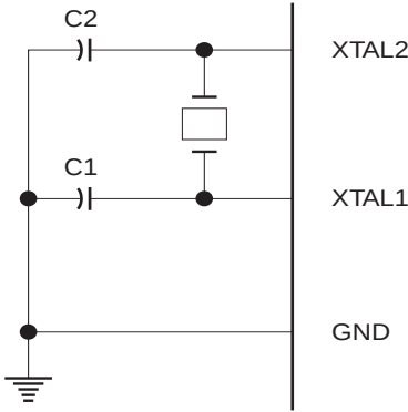
Figure 1. Oscillator Connections
