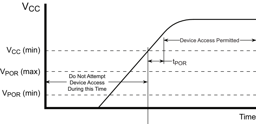
Figure 8-2. Power-Up Timing
