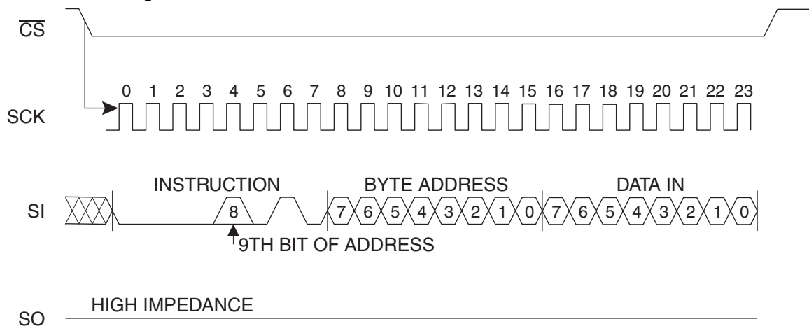
Figure 6-7. WRITE Timing
