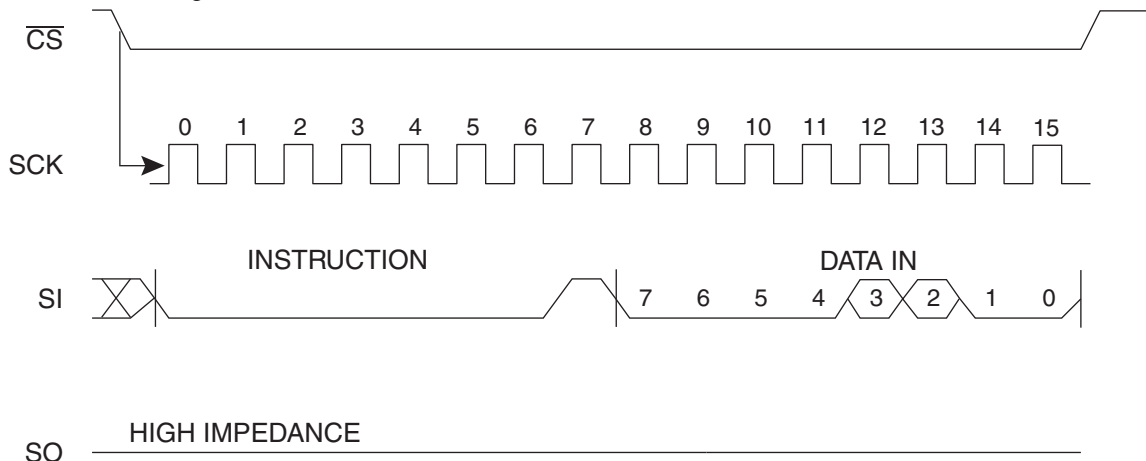
Figure 6-5. WRSR Timing
