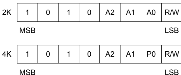
Figure 7-1. Device Address
