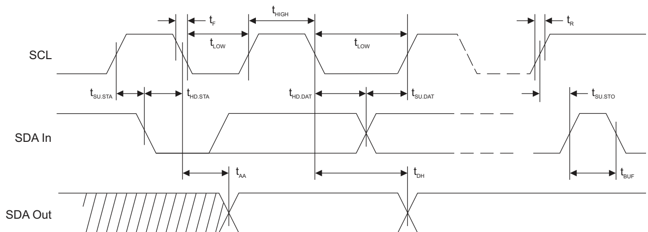
Figure 6-5. Bus Timing
