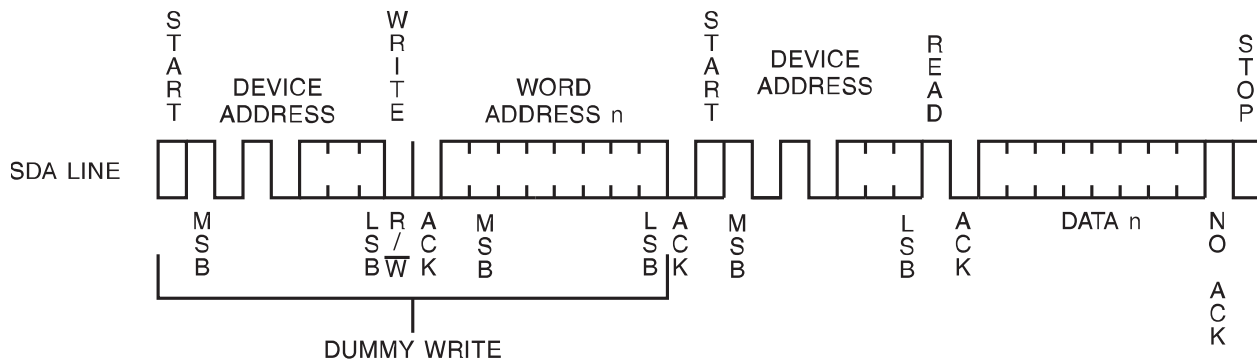
Figure 13. Random Read
