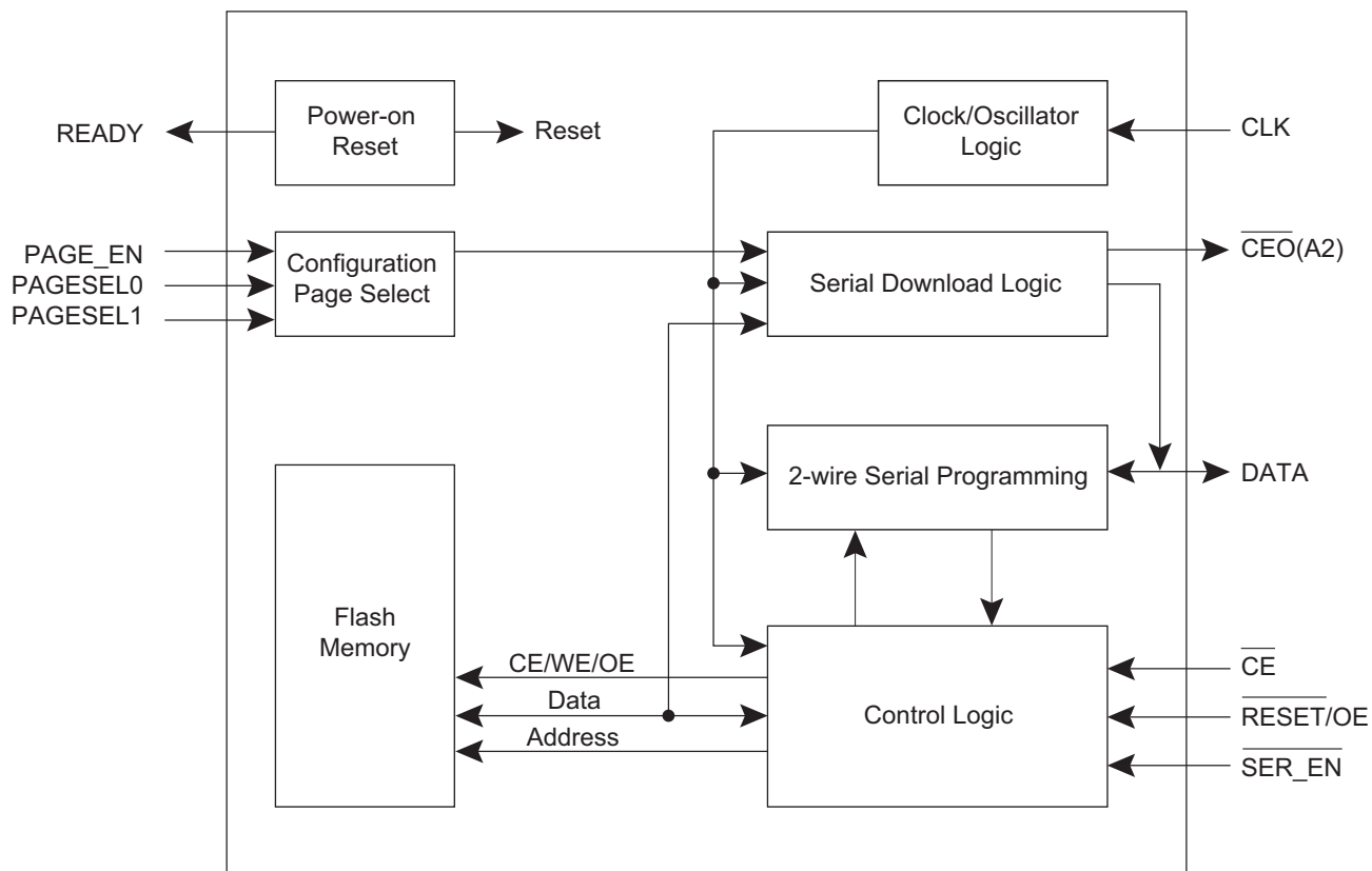
Figure 2-1. Block Diagram
