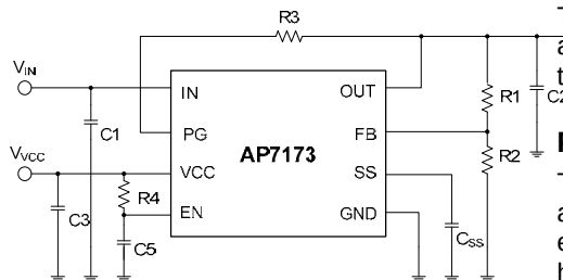
Figure 30. Delayed Start Using an RC Circuit to Enable AP7173
