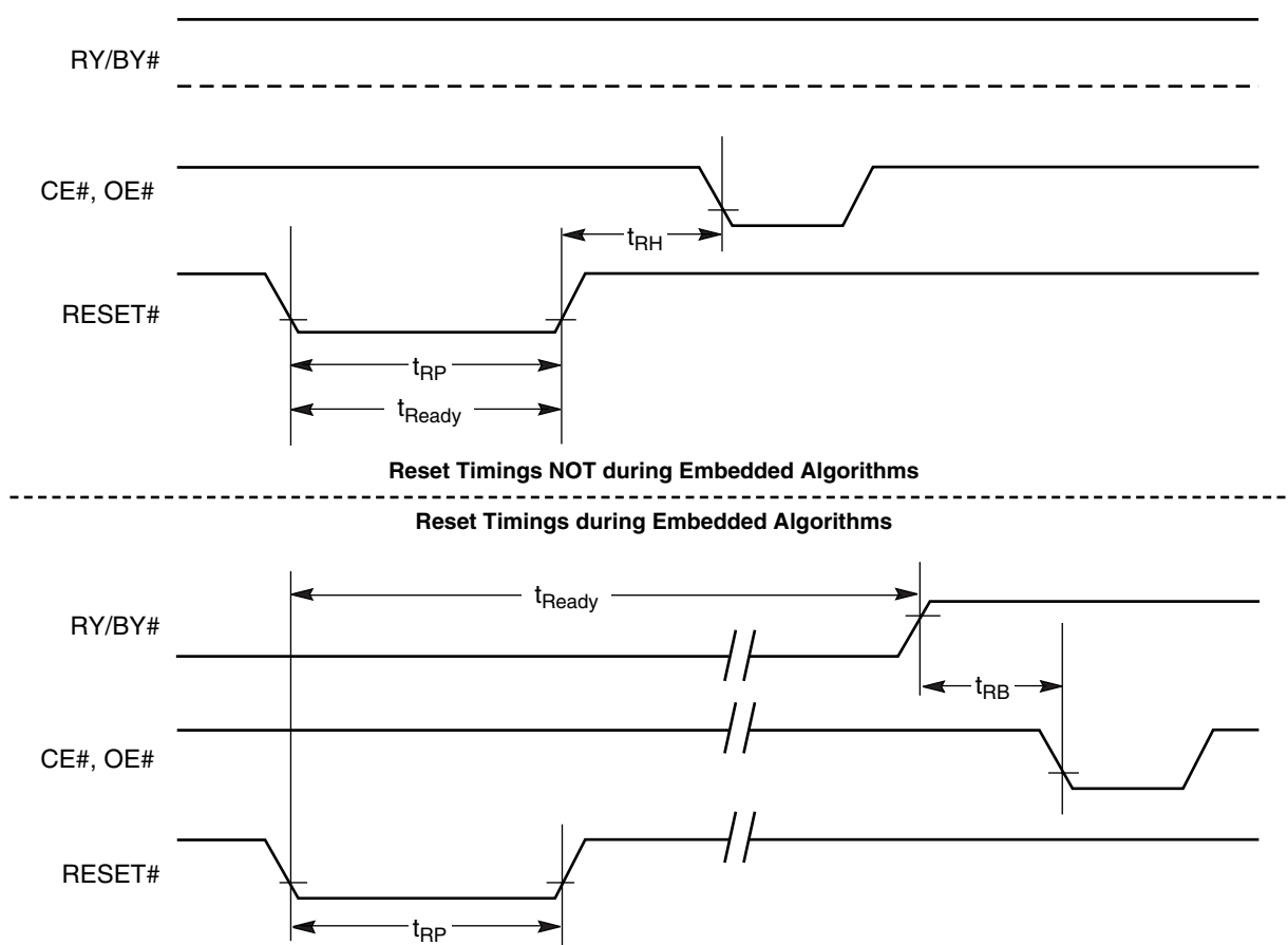
Figure 10. RESET# Timings
