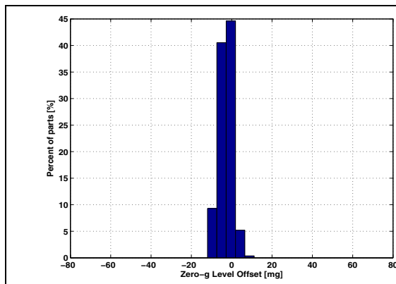
Figure 21. Z-axis zero-g level at 3.3 V
