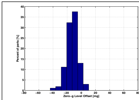
Figure 19. Y-axis zero-g level at 3.3 V
