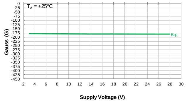
Switch Release Point B_{rp} vs Supply Voltage
