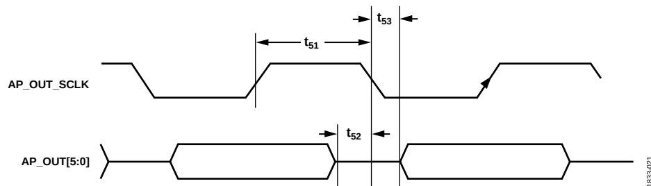
Figure 18. DSD Output Timing
