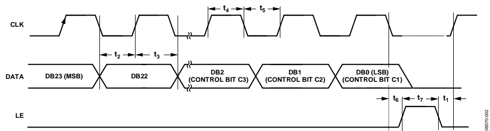
Figure 2. Timing Diagram
