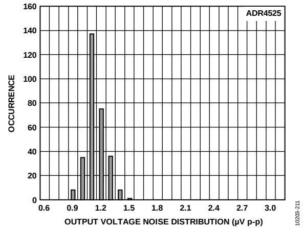
Figure 27. ADR4525 Output Voltage Noise (Maximum Amplitude from 0.1 Hz to 10 Hz)
