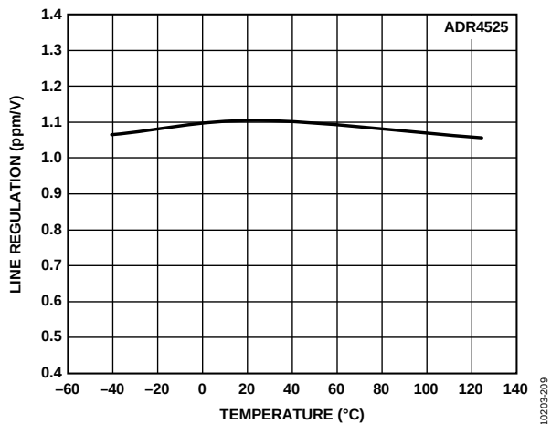
Figure 25. ADR4525 Line Regulation vs. Temperature
