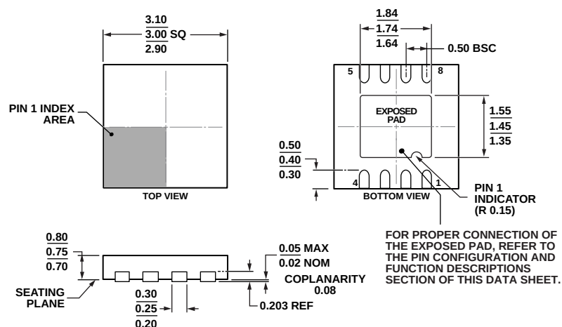
Figure 26. 8-Lead Lead Frame Chip Scale Package [LFCSF_WD] 3 mm × 3 mm Body, Very Very Thin, Dual Lead (CP-8-13)
