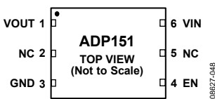
Figure 6. 6-Lead LFCSP Pin Configuration
