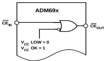
Figure 5. Chip Enable Gating
