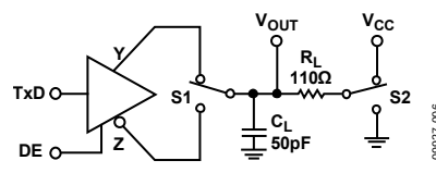
Figure 32. Driver Enable/Disable
