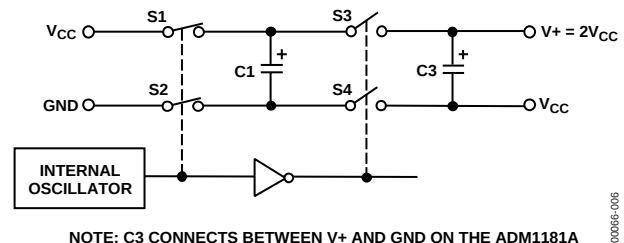
Figure 6. Charge-Pump Voltage Doubler
