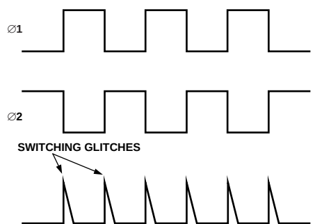
Figure 24. Switching Glitches
