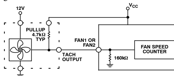
Figure 25. Fan with Tach Pullup to + V_{CC}
