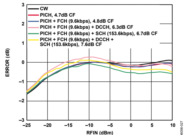
Figure 27. Error from CW Linear Reference vs. Input with Various CDMA2000 Reverse Link Waveforms at 900 MHz, C_{FILT} = 1 nF, C_{OUT} = 100 nF
