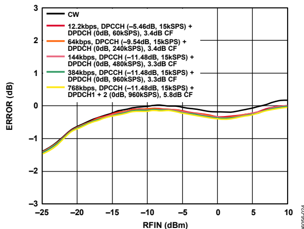
Figure 24. Error from CW Linear Reference vs. Input with Various WCDMA Up Link Waveforms at 1900 MHz, C_{FILT} = Open, C_{OUT} = 100 nF
