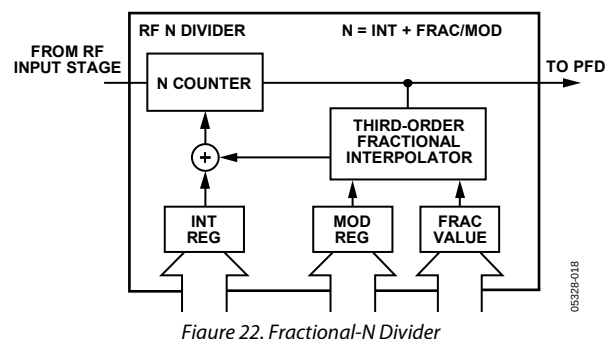
Figure 22. Fractional-N Divider
