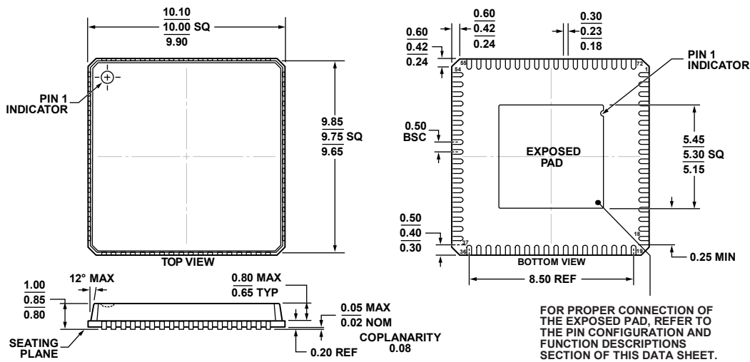
Figure 91. 72-Lead Lead Frame Chip Scale Package [LFCSP_VQ] 10 mm x 10 mm Body, Very Thin Quad (CP-72-6) Dimensions shown in millimeters
