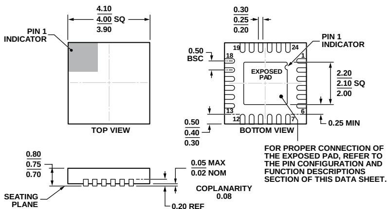
Figure 72. 24-Lead Lead Frame Chip Scale Package [LFCSP] 4 mm × 4 mm Body, and 0.75 mm Package Height (CP-24-10)
