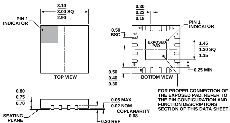
Figure 71. 16-Lead Lead Frame Chip Scale Package [LFCSP] 3 mm × 3 mm Body and 0.75 mm Package Height (CP-16-21)
