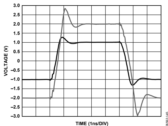
Figure 46. Large Signal Transient Response
