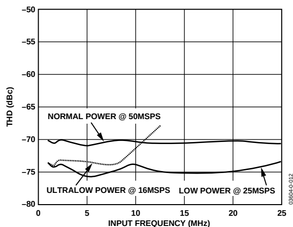
Figure 15. AD9863 Rx Path at 50 MSPS, 10 MHz Input Tone THD Performance vs. Input Frequency
