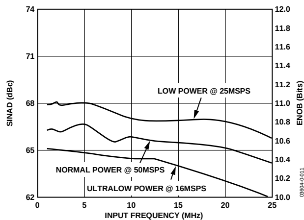
Figure 14. AD9863 Rx Path at 50 MSPS, 10 MHz Input Tone SINAD Performance vs. Input Frequency
