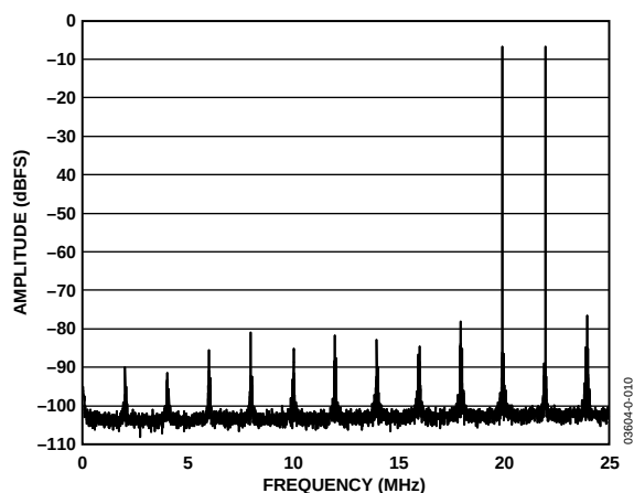
Figure 13. AD9863 Rx Path Dual-Tone FFT of Rx Channel A Path Digitizing 70 MHz and 72 MHz Tones
