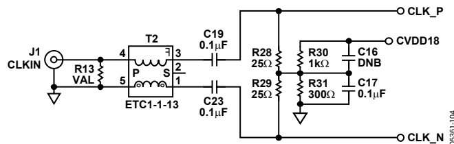
Figure 107. Evaluation Board, Rev. D, DAC Clock Interface
