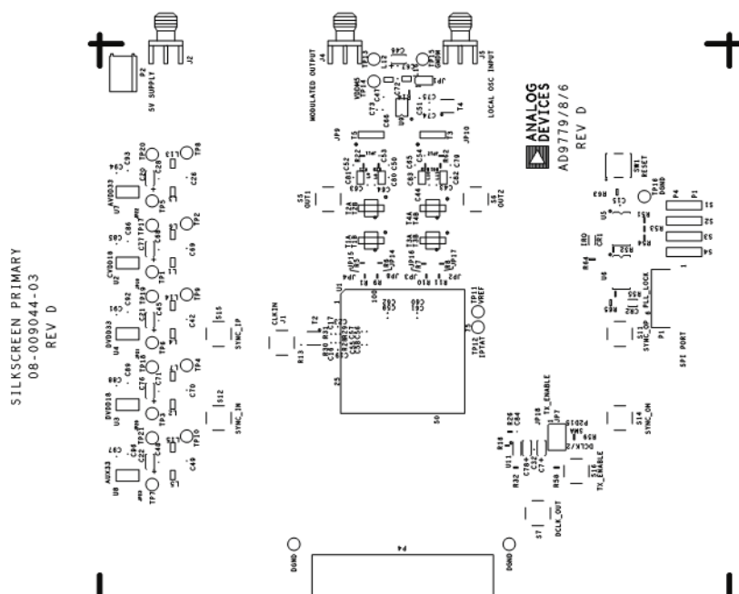
Figure 110. Evaluation Board, Rev. D, Top Silk Screen
