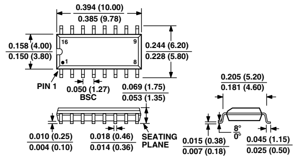
16-Lead SOIC
