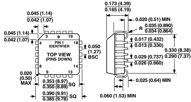
20-Lead PLCC
