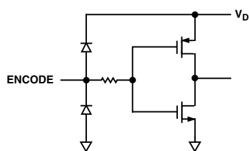
Figure 4. Equivalent Encode Input Circuit
