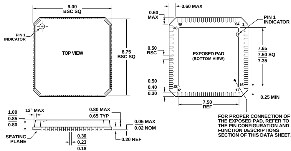
COMPLIANT TO JEDEC STANDARDS MO-220-VMMD-4 Figure 85. 64-Lead Lead Frame Chip Scale Package [LFCSP_VQ] 9 mm x 9 mm Body, Very Thin Quad (CP-64-6) Dimensions shown in millimeters
