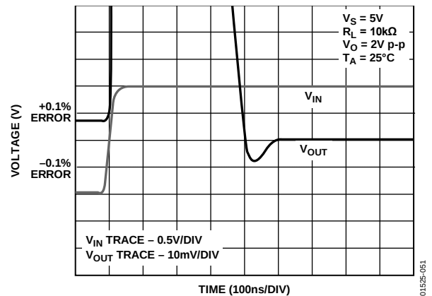
Figure 51. Settling Time
