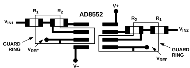
Figure 53. Top View of AD8552 SOIC Layout with Guard Rings
