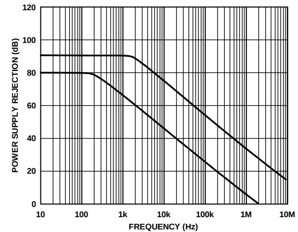
Figure 22. Power Supply Rejection vs. Frequency
