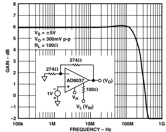
TPC 30. AD8037 Clamp Input Bandwidth, V_H , V_L
