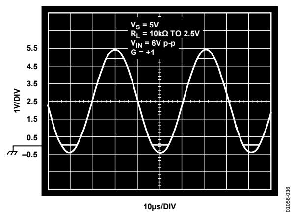
Figure 36. Output Voltage
