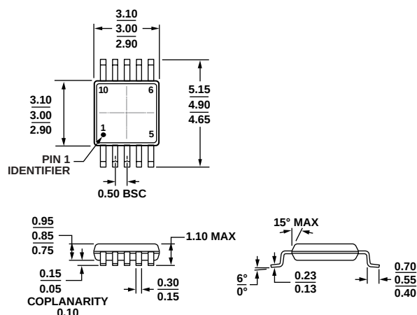
COMPLIANT TO JEDEC STANDARDS MO-187-BA Figure 71. 10-Lead Mini Small Outline Package [MSOP] (RM-10) Dimensions shown in millimeters
