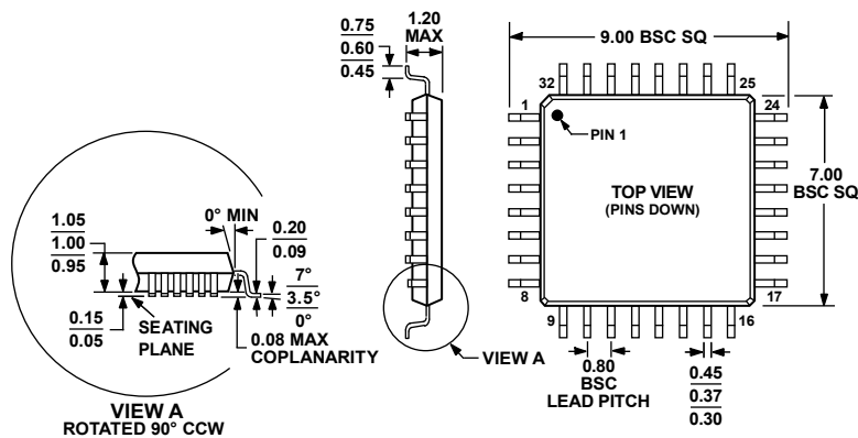
Figure 48. 32-Lead Thin Plastic Quad Flat Package [TQFP]
