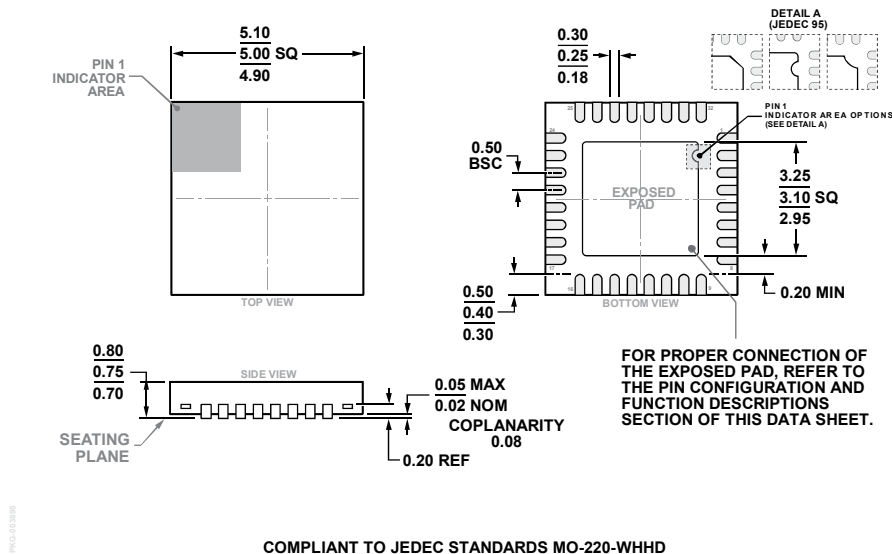
Figure 47. 32-Lead Lead Frame Chip Scale Package [LFCSP]
